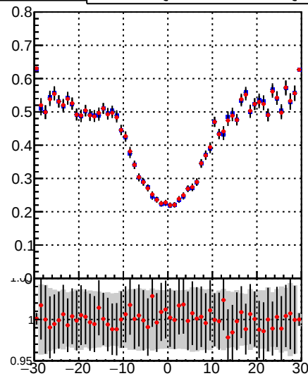
—•— DQM_TT_mkFit-DQM_original —•— DQM_TT_mkFit-DQM_modified5
