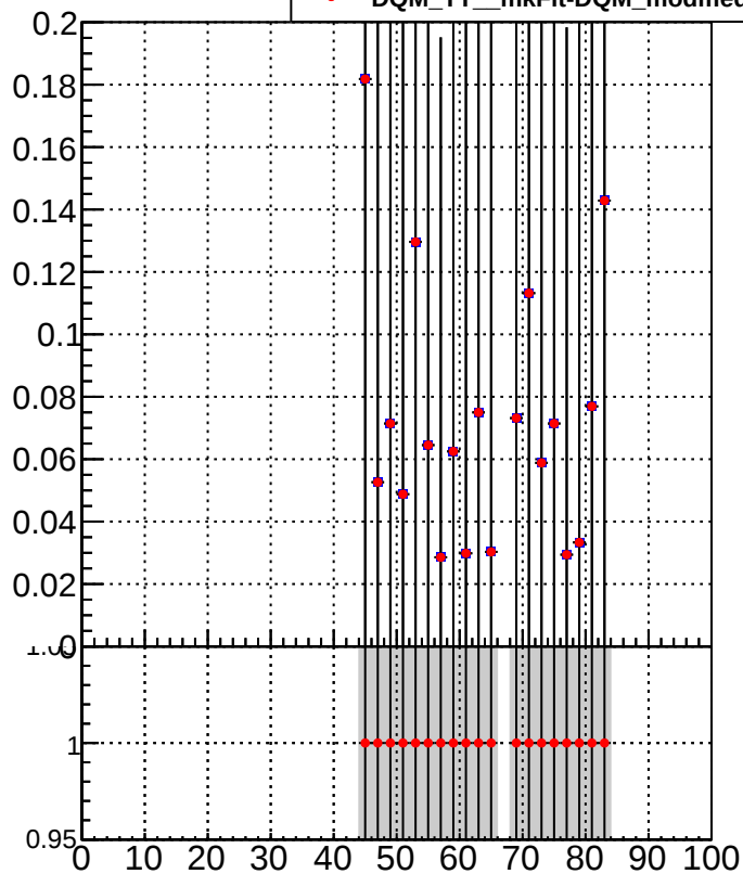
■ DQM_TT_mkFit-DQM_original ● DQM_TT_mkFit-DQM_modified5
