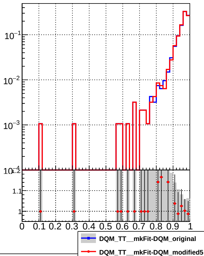
RecoPVAssoc2GenPVMatched_Missing
