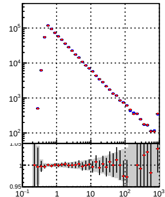
—•— DQM_TT_mkFit-DQM_original —•— DQM_TT_mkFit-DQM_modified5
