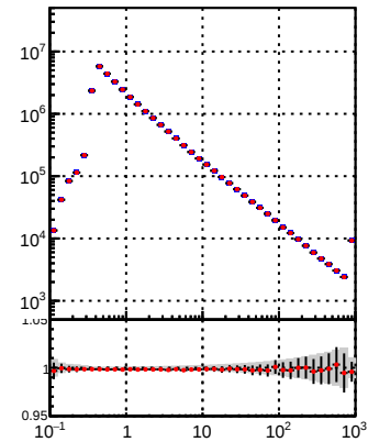
—●— DQM_TT mkFit-DQM_original —●— DQM_TT mkFit-DQM_modified5
