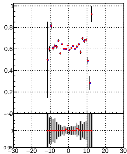
—•— DQM_TT_mkFit-DQM_original —•— DQM_TT_mkFit-DQM_modified5
