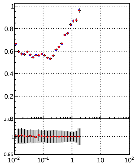
—•— DQM_TT_mkFit-DQM_original —•— DQM_TT_mkFit-DQM_modified5
