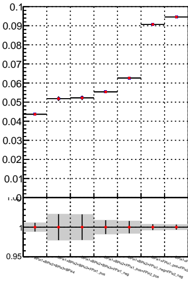
Fake rate vs. —■— DQM_TT_mkFit-DQM_original —●— DQM_TT_mkFit-DQM_modified5
