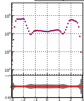
N of reco track vs \eta DQM_TT_mkFit-DQM_original DQM_TT_mkFit-DQM_modified5
