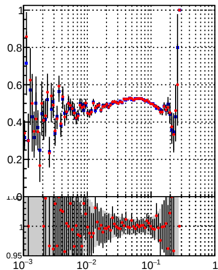
—•— DQM_TT_mkFit-DQM_original —•— DQM_TT_mkFit-DQM_modified5
