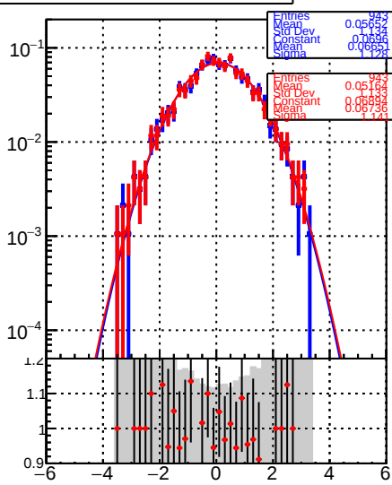
RecoPVAssoc2GenPVMatched_PulIX
