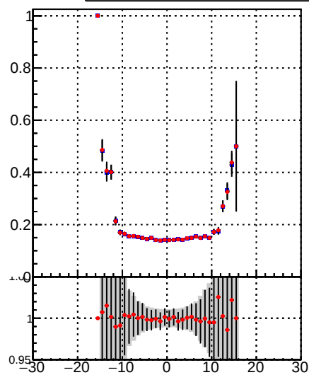
—•— DQM_TT_mkFit-DQM_original —•— DQM_TT_mkFit-DQM_modified5
