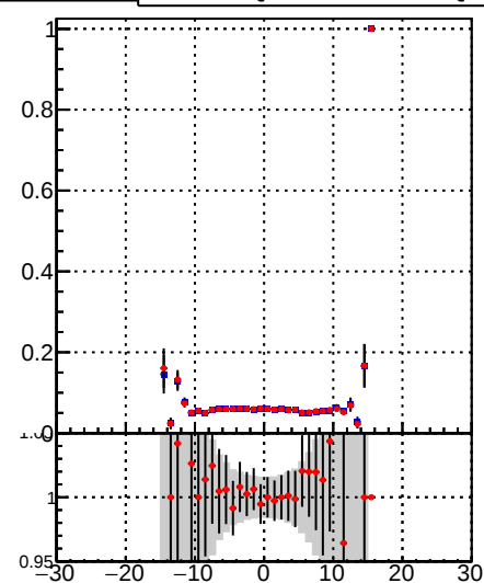
—•— DQM_TT_mkFit-DQM_original —•— DQM_TT_mkFit-DQM_modified5
