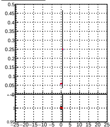
—●— DQM_TT_mkFit-DQM_original —●— DQM_TT_mkFit-DQM_modified5
