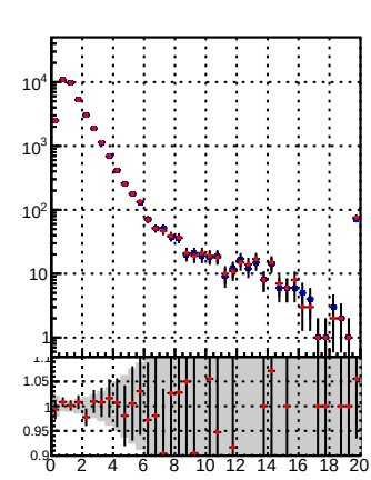
Legend: - DQM TT mkFit-DQM_original (blue line with circles) - DQM TT mkFit-DQM_modified5 (red line with circles) - verSet (gray bars)
