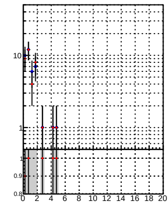
Legend: - DQM TT mkFit-DQM_original (blue line with circles) - DQM TT mkFit-DQM_modified5 (red line with circles) - verSet (gray bars)
