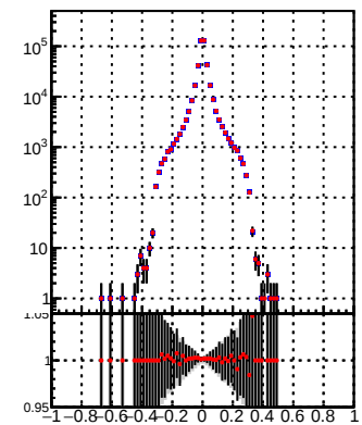
DQM_TT_mkFit-DQM_original DQM_TT_mkFit-DQM_modified5
