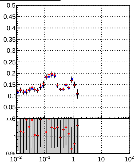
—•— DQM_TT_mkFit-DQM_original —•— DQM_TT_mkFit-DQM_modified5
