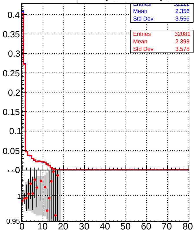
Legend: DQM_TT_mkFit-DQM_original DQM_TT_mkFit-DQM_modified5
