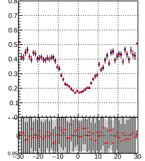
Efficiency vs. sim PV z Legend: — DQM_TT_mkFit-DQM_original — DQM_TT_mkFit-DQM_modified5
