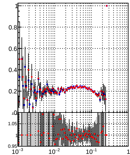
Legend: DQM_TT_mkFit-DQM_original (blue squares) DQM_TT_mkFit-DQM_modified5 (red circles)
