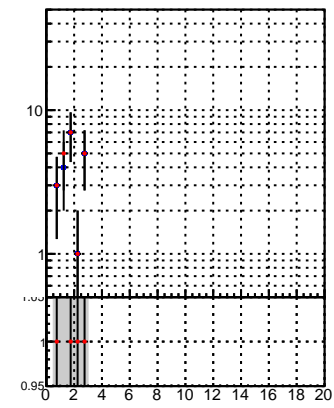
N of reco track vs. s DQM_TT mkFit-DQM_original DQM_TT mkFit-DQM_modified5
