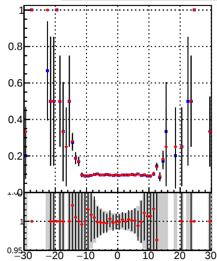
—•— DQM_TT_mkFit-DQM_original —•— DQM_TT_mkFit-DQM_modified5
