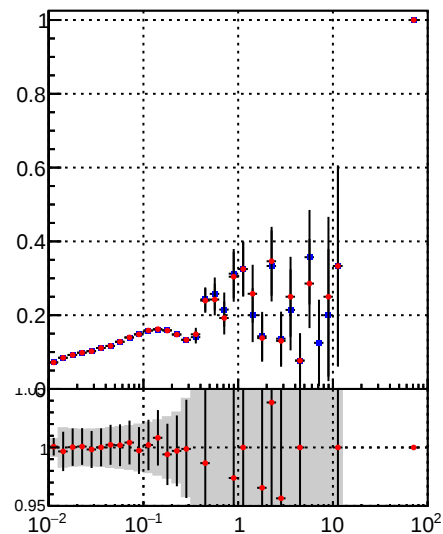
—•— DQM_TT_mkFit-DQM_original —•— DQM_TT_mkFit-DQM_modified5
