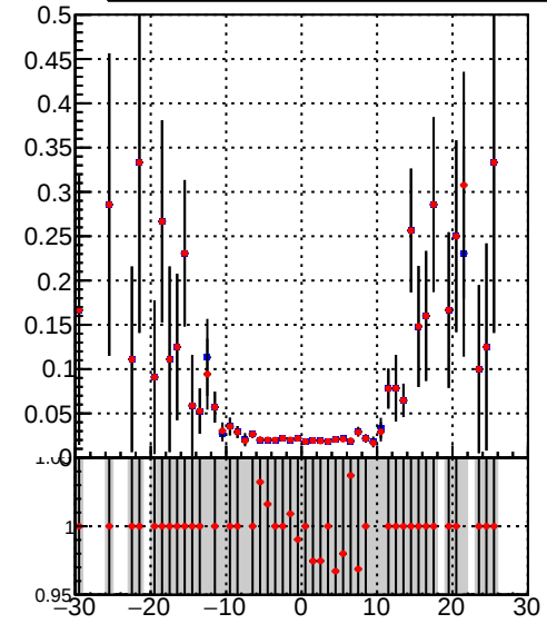
Efficiency vs. sim PV z Legend: DQM_TT_mkFit-DQM_original (blue circles) DQM_TT_mkFit-DQM_modified5 (red circles)
