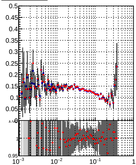
— DQM_TT_mkFit-DQM_original — DQM_TT_mkFit-DQM_modified5
