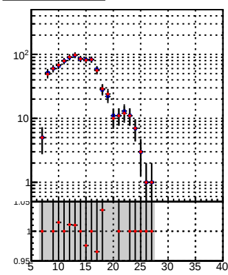
DQM_TT_mkFit-DQM_original DQM_TT_mkFit-DQM_modified5
