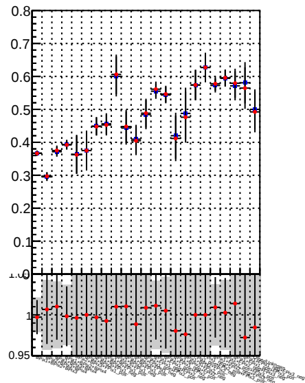
Fake rate vs. —●— DQM_TT_mkFit-DQM_original —●— DQM_TT_mkFit-DQM_modified5
