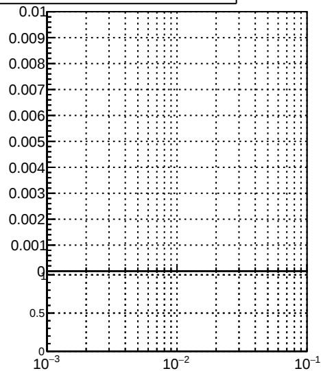
Pileup rate vs r
