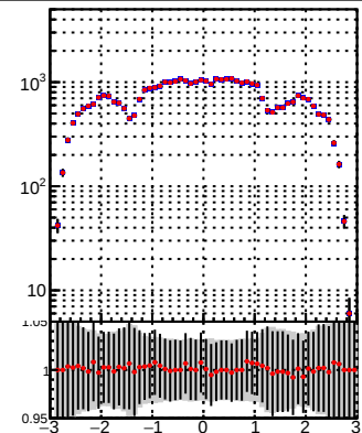
—●— DQM_TT_mkFit-DQM_original —●— DQM_TT_mkFit-DQM_modified5
