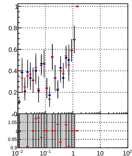
—•— DQM_TT_mkFit-DQM_original —•— DQM_TT_mkFit-DQM_modified5
