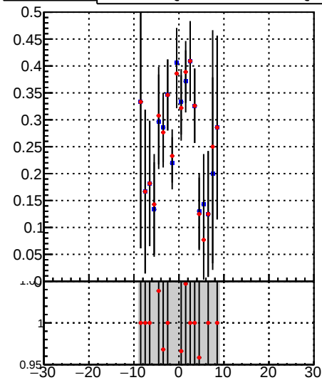
—•— DQM_TT_mkFit-DQM_original —•— DQM_TT_mkFit-DQM_modified5
