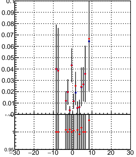
Efficiency vs vert r —■— DQM_TT_mkFit-DQM_original —●— DQM_TT_mkFit-DQM_modified5
