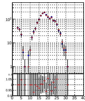
—•— DQM_TT_mkFit-DQM_original —•— DQM_TT_mkFit-DQM_modified5
