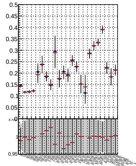
Fake rate vs. DQM_TT_mkFit-DQM_original DQM_TT_mkFit-DQM_modified5
