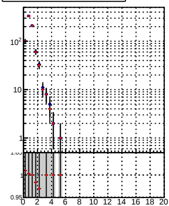
N of reco track vs. \chi^2 mkFit-DQM_original mkFit-DQM_modified5
