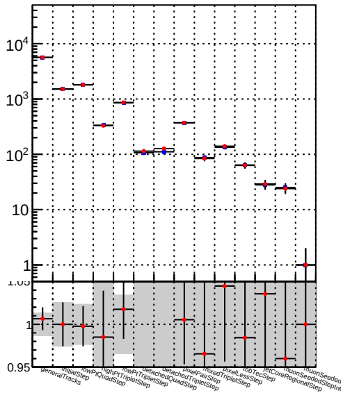
Number —●— DQM_TT__mkFit-DQM_modified5
