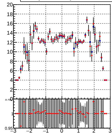
mean hit — DQM_TT_mkFit-DQM_original — DQM_TT_mkFit-DQM_modified5
