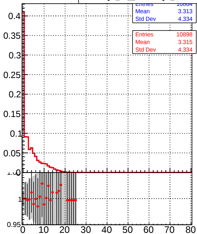
Legend: DQM_TT_mkFit-DQM_original (Blue line with squares) DQM_TT_mkFit-DQM_modified5 (Red line with circles)
