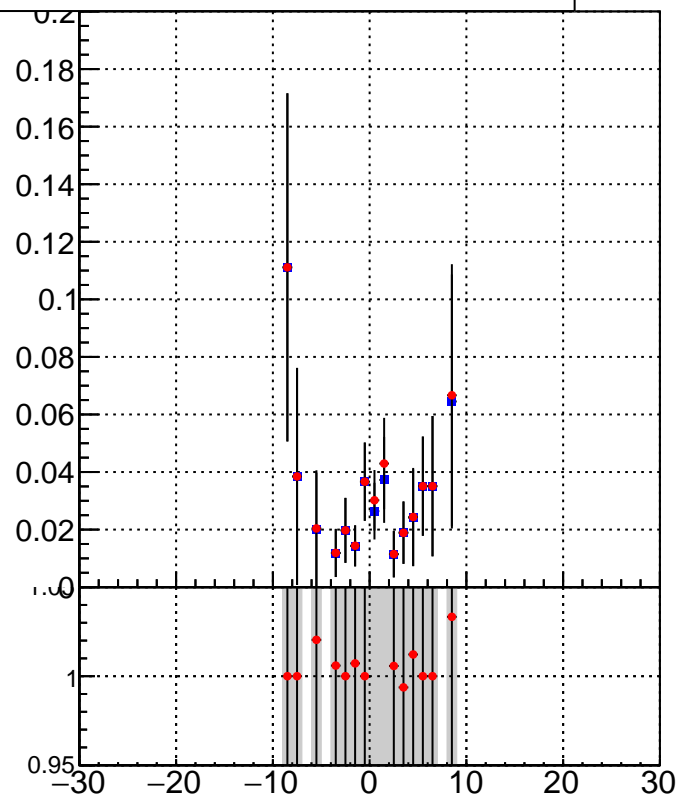
DQM_TT_mkFit-DQM_original DQM_TT_mkFit-DQM_modified5
