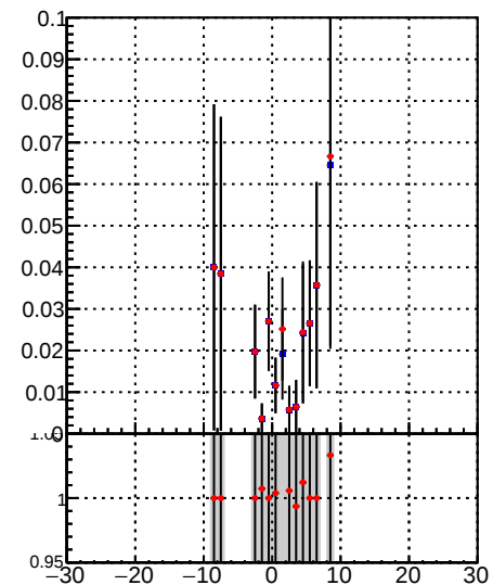
—●— DQM_TT_mkFit-DQM_original —●— DQM_TT_mkFit-DQM_modified5
