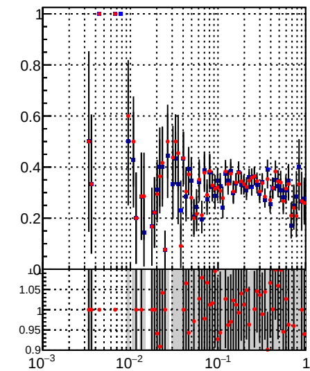
—•— DQM_TT_mkFit-DQM_original —•— DQM_TT_mkFit-DQM_modified5
