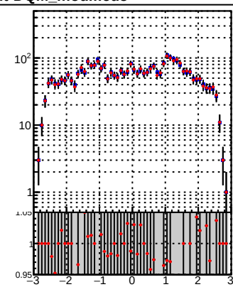
—●— DQM_TT_mkFit-DQM_original —●— DQM_TT_mkFit-DQM_modified5
