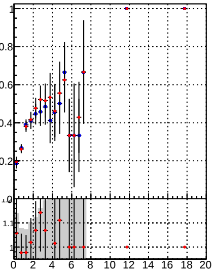
Fake rate vs. —●— DQM_TT_mkFit-DQM_original —●— DQM_TT_mkFit-DQM_modified5
