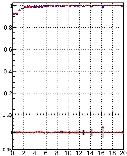
Fake rate vs. DQM_TT_mkFit-DQM_original DQM_TT_mkFit-DQM_modified5
