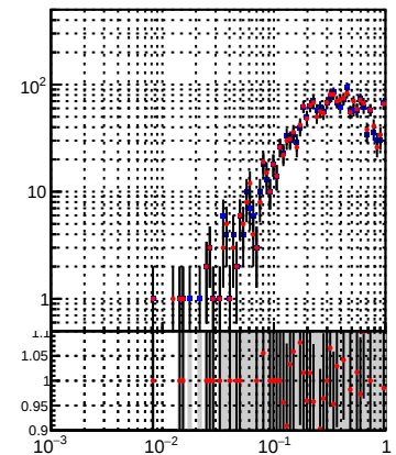
N of associated tracks (recoToSim) vs dR
