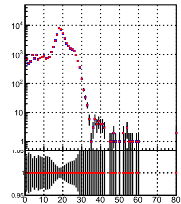
■ DQM_TT_mkFit-DQM_original ■ DQM_TT_mkFit-DQM_modified5
