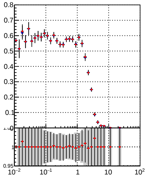
Efficiency vs vert r Legend: DQM_TT_mkFit-DQM_original (blue diamonds) DQM_TT_mkFit-DQM_modified5 (red diamonds)
