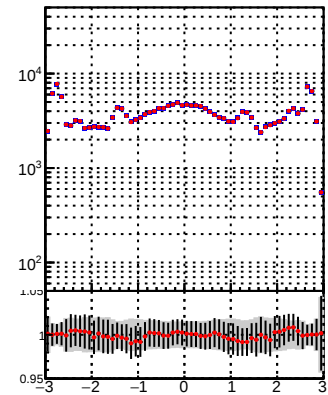
N of reco track vs \eta Legend: —•— DQM_TT_mkFit-DQM_original —•— DQM_TT_mkFit-DQM_modified5
