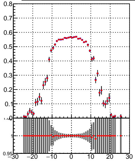
Efficiency vs vert r — DQM_TT_mkFit-DQM_original (blue squares) — DQM_TT_mkFit-DQM_modified5 (red stars)
