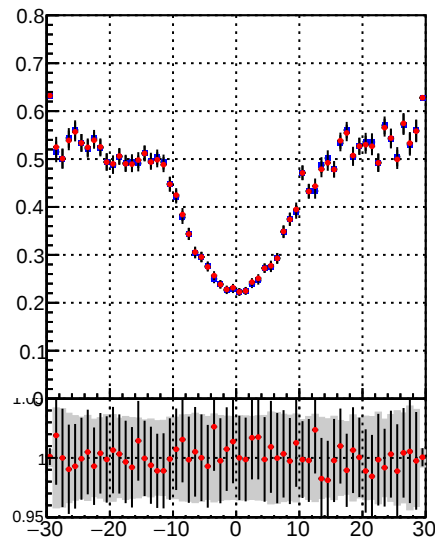
Fake rate vs d —●— DQM\_TT\_mkFit-DQM\_original —●— DQM\_TT\_mkFit-DQM\_modified5
