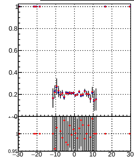
—•— DQM_TT_mkFit-DQM_original —•— DQM_TT_mkFit-DQM_modified5
