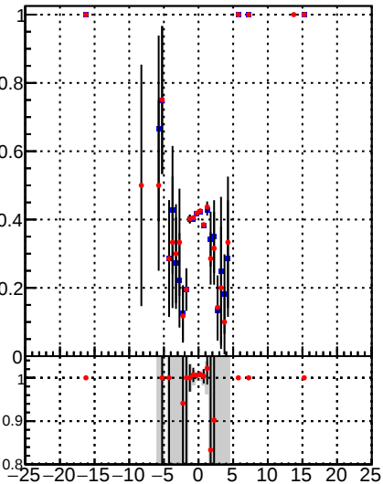
Fake rate vs d —•— DQM_TT_mkFit-DQM_original —•— DQM_TT_mkFit-DQM_modified5
