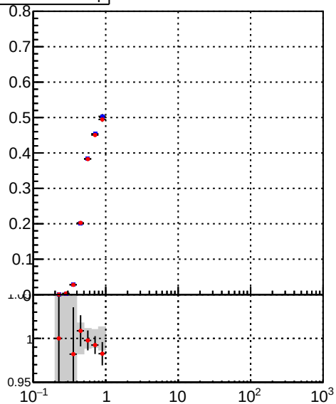
Legend: —■— DQM_TT_mkFit-DQM_original —●— DQM_TT_mkFit-DQM_modified4
